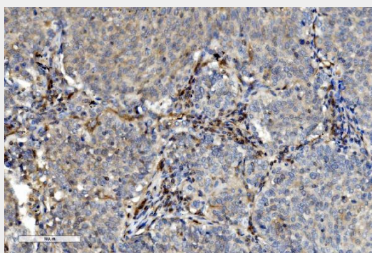
Figure 2. IHC analysis of PNP using anti-PNP antibody (M00988).
