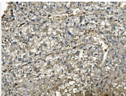
Figure 3. IHC analysis of PNP using anti-PNP antibody (M00988).
