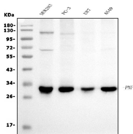
Figure 1. Western blot analysis of PNP using anti-PNP antibody (M00988).
