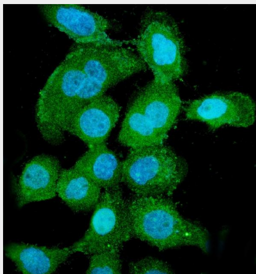
Figure 4. IF analysis of PNP using anti-PNP antibody (M00988).
